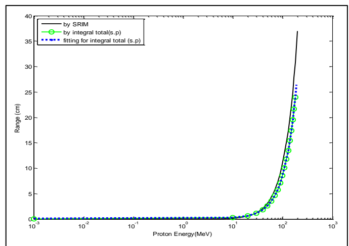
Figure 2. Range of Proton in Lymph Tissue
